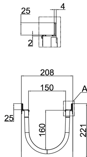
Detalle A (2:1)
